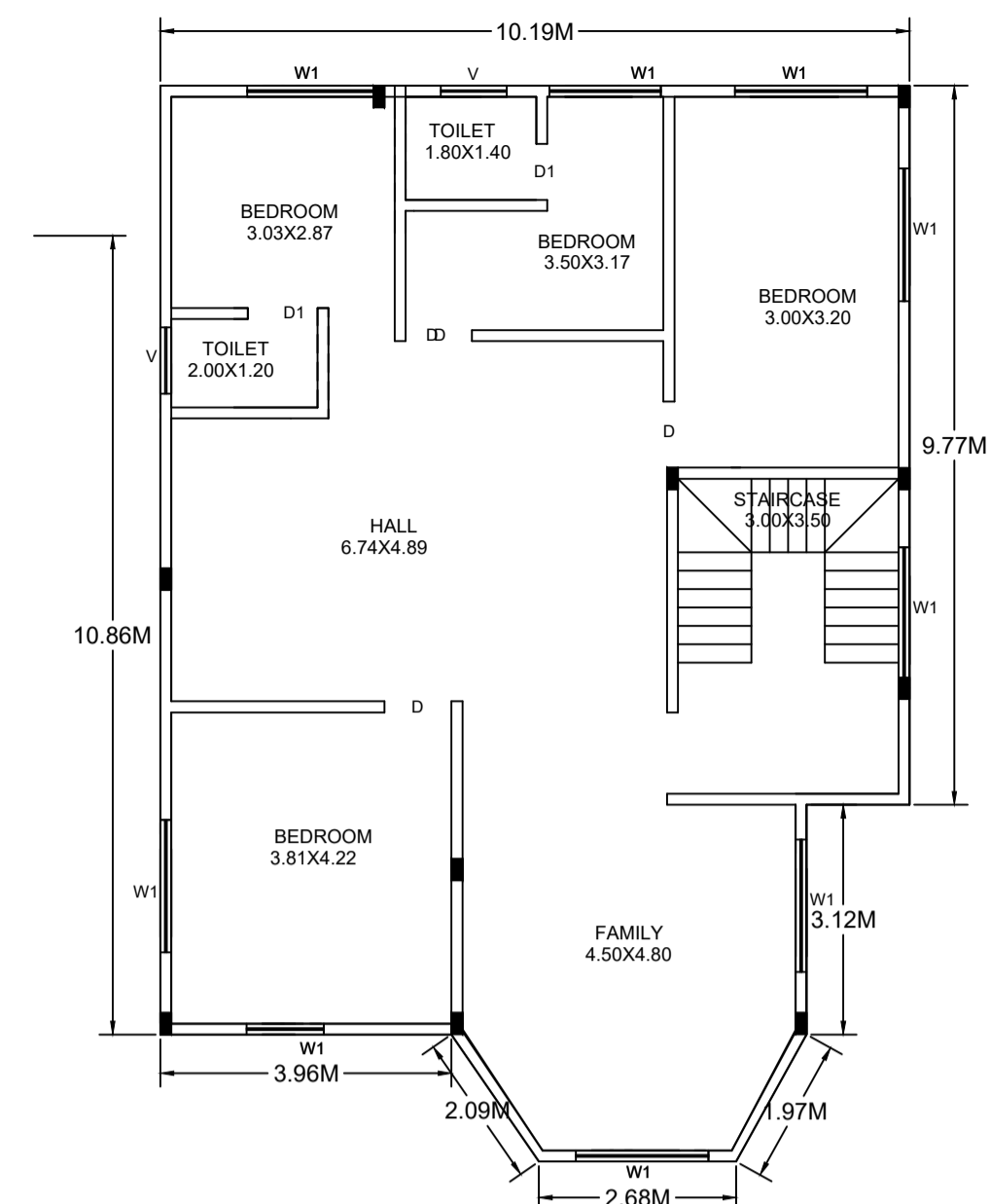
EX. FIRST FLOOR PLAN
